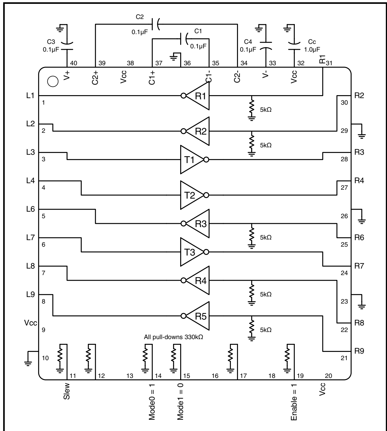
FIGURE 2. MODE 01 - RS-232
