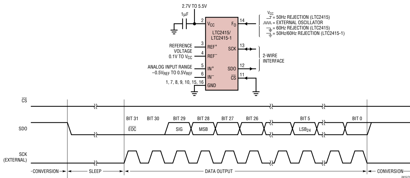
Figure 10. External Serial Clock, \overline{\text{CS}} = 0 Operation (2-Wire)
