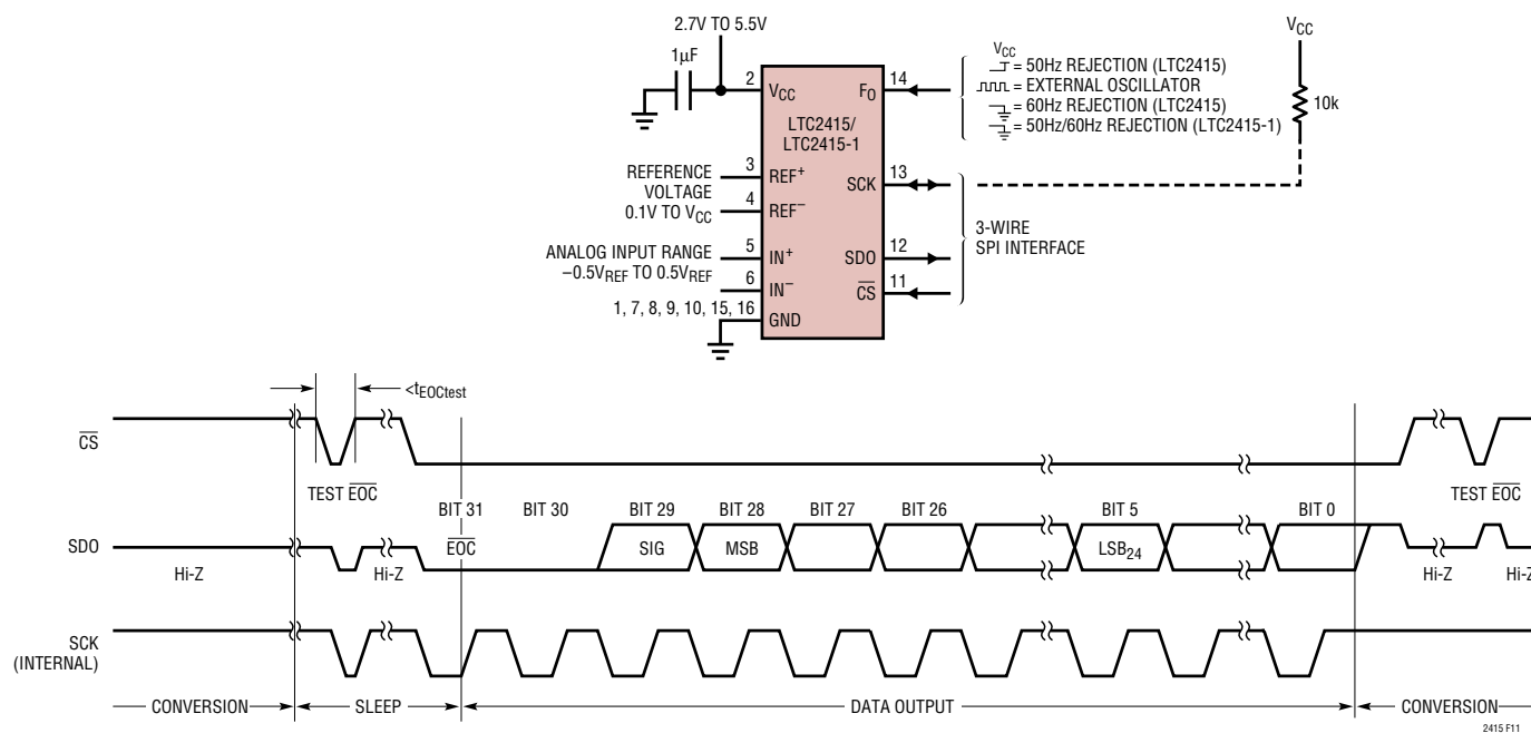
Figure 11. Internal Serial Clock, Single Cycle Operation
