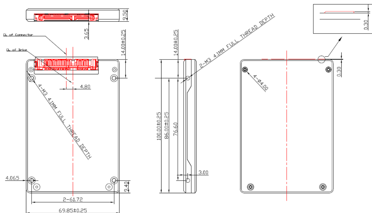
Figure 2-1. Physical dimension
