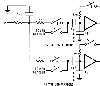
Figure 27. ADC0820-N Input Circuit
