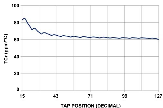
FIGURE 18. 100kΩ TCcr vs TAP POSITION, V_{CC} = 3.3V
