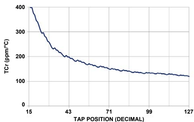
FIGURE 15. 10kΩ TCcr vs TAP POSITION
