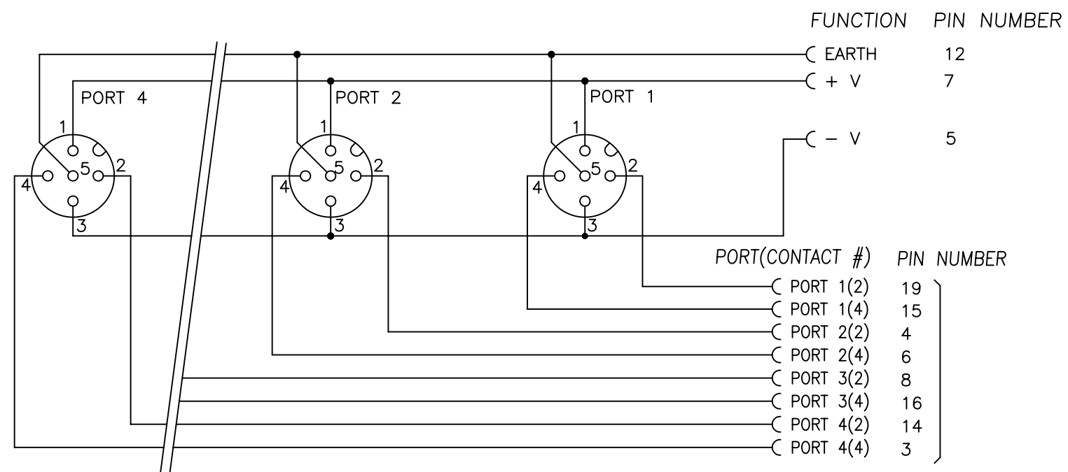
FACE VIEW OF END RECEPTACLE
