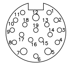
FACE VIEW OF END RECEPTACLE
