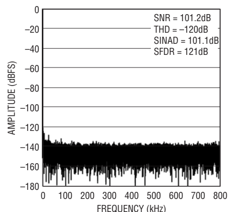
32k Point FFT f_{\text{S}} = 1.6\text{Msps} , f_{\text{IN}} = 2\text{kHz}
