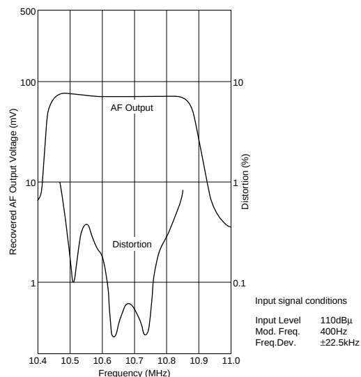
Frequency Characteristics
