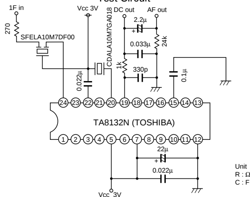
Test Circuit
