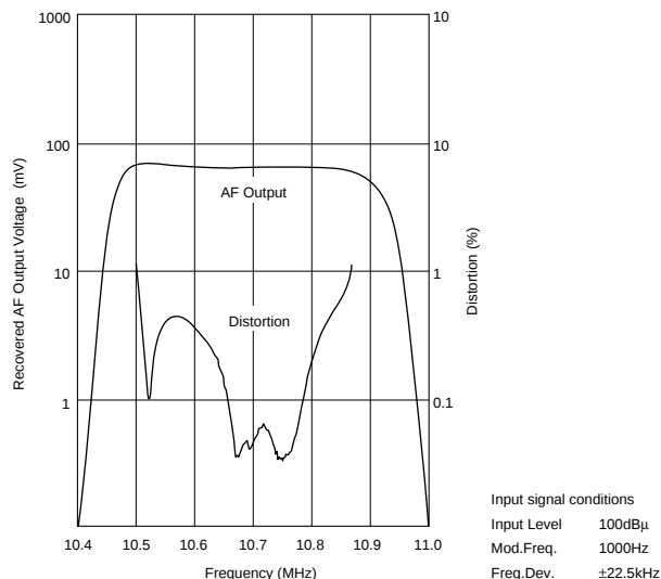
Frequency Characteristics
