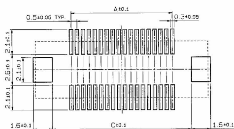
MOUNTING LAYOUT
