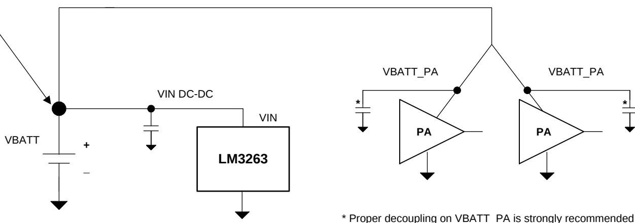
Star Connection at VBATT
