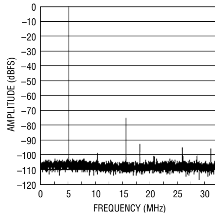
Averaged 8192 Point FFT, Input Frequency = 70MHz, -1dB, 3.2V Range
