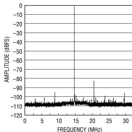
Averaged 8192 Point FFT, Input Frequency = 50MHz, -1dB, 3.2V Range
