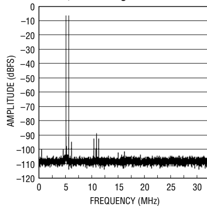
Averaged 8192 Point 2-Tone FFT, 5.2MHz and 5.7MHz Inputs, -7dB, 3.2V Range
