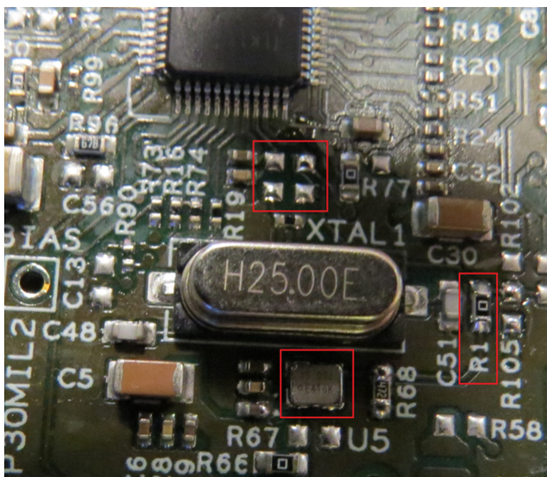
Figure 9. 25M OSC Modifications
