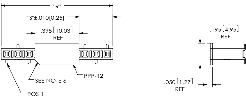
FIG 6 -P: PICK AND PLACE PAD (SSM-110-XXX-SV-P SHOWN) -02 AND -03 POS NOT AVAILABLE WITH POLARIZATION -04 POS - CANNOT OFFER IF POLARIZATION IS POS 2 OR 3 -05 POS - CANNOT OFFER IF POLARIZATION IS POS 3 *MUST USE TR ON POS 2 & 3 (DIFFERENT AS SHOWN, OTHERWISE SAME AS FIG 1) "R" = SEE FIG 1, SHEET 1 FOR OAL "S" = IF NO OF POS IS EVEN: "R"/2 - .1975 [5.017] IF NO OF POS IS ODD: "R"/2 - .2475 [6.287]
