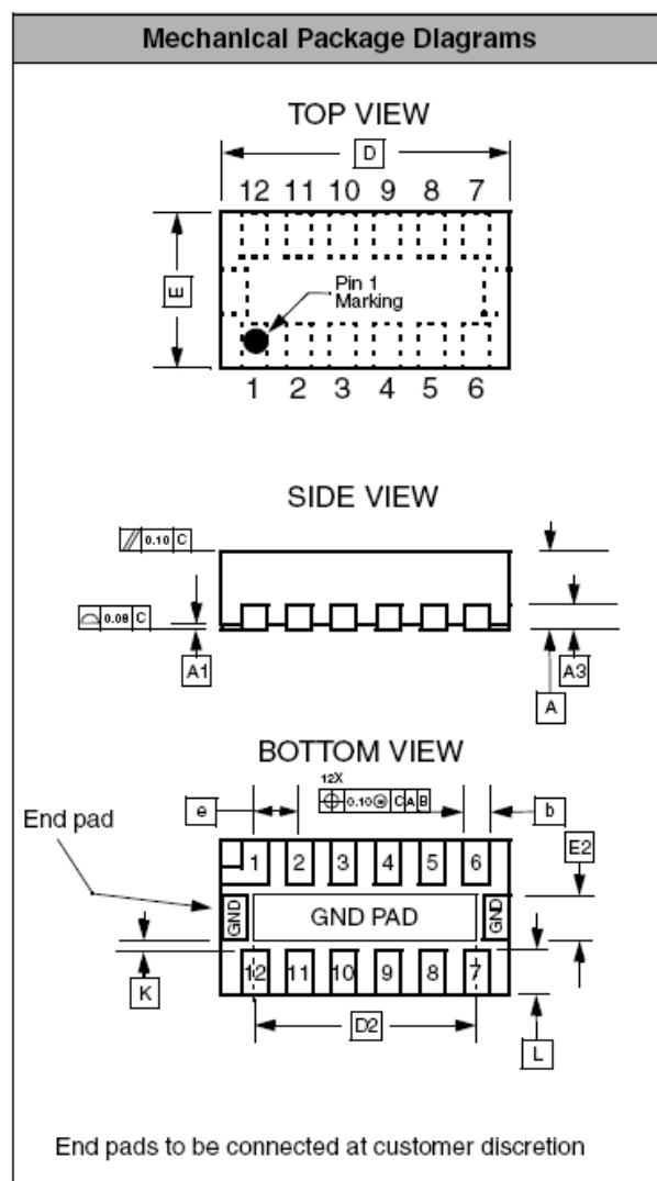
Dimensions for 12-Lead, 0.4mm pitch NuDFN package
