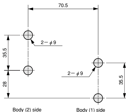
Layout of Holes for Installation
