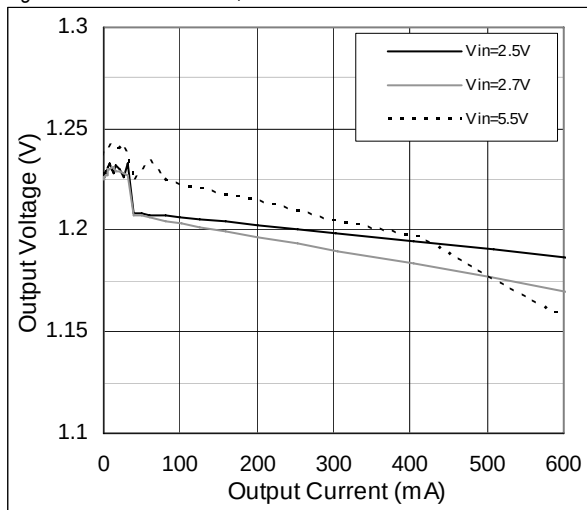
Figure 13. VOUT vs. IOUT; VOUTNOM = 1.2V
