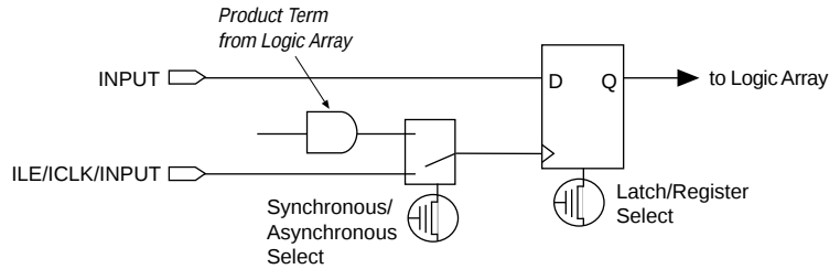
Figure 4. EP312 & EP324 Input Structure
