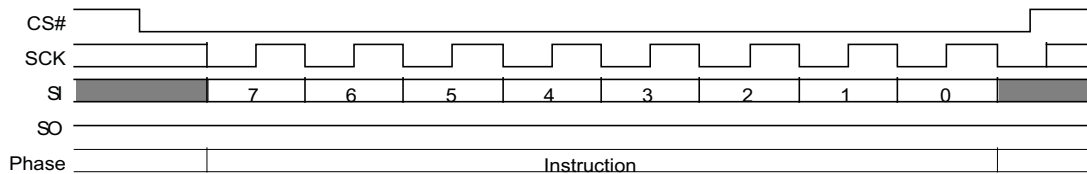
Figure 56. BRAC (B9h) Command Sequence
