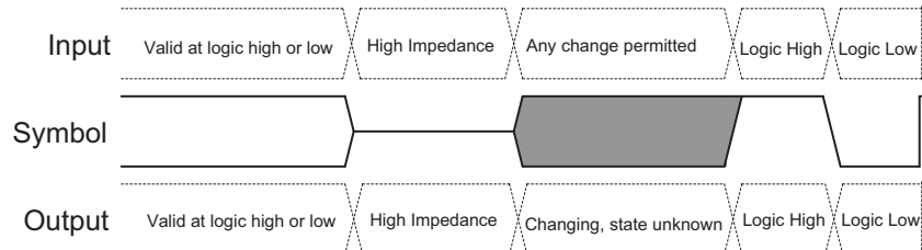
Figure 23. Waveform Element Meanings
