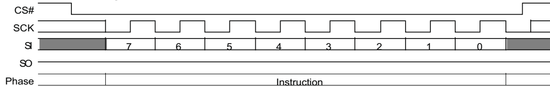
Figure 121. Mode Bit (MBR FFh) Reset Command Sequence
