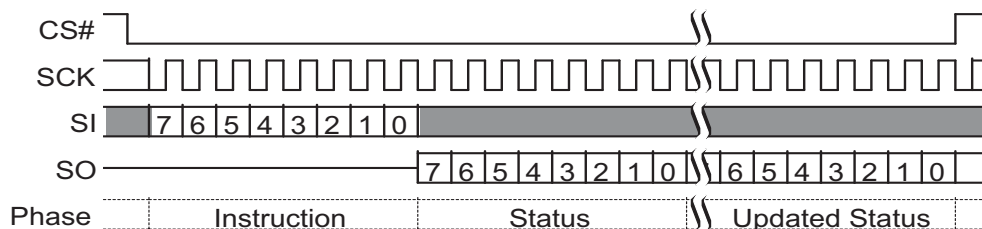
Figure 52. Read Status Register-2 (RDSR2 07h) Command Sequence
