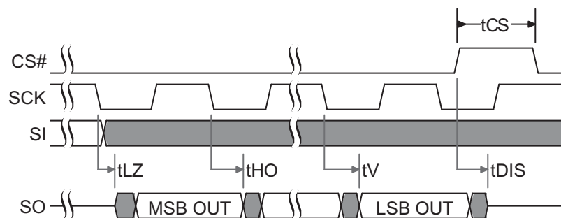
Figure 32. SPI Single Bit Output Timing
