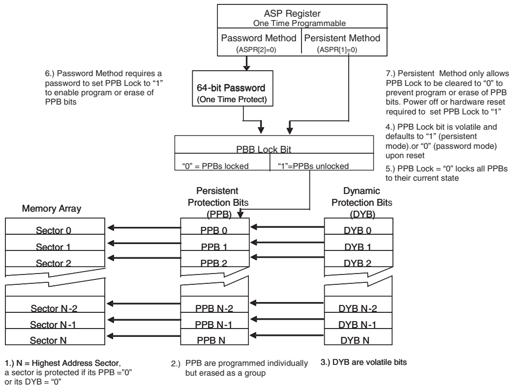
Figure 46. Advanced Sector Protection Overview
