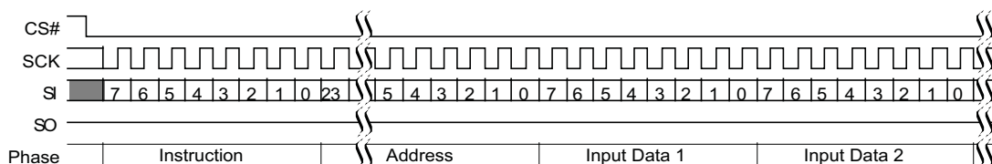
Figure 106. Page Program (OTPP 42h) Command Sequence
