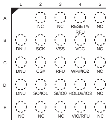
Figure 41. 24-Ball BGA, 5 x 5 Ball Footprint (FAB024), Top View
