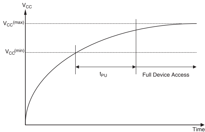
Figure 21. Power-Up
