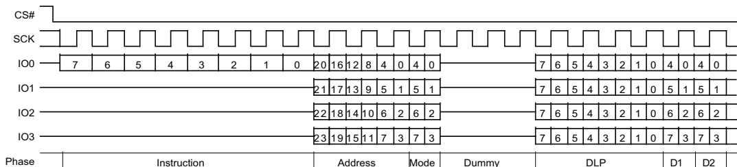
Figure 95. Continuous DDR Quad I/O Read Subsequent Access (3-Byte Address, HPLC=11b)
