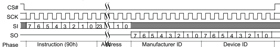
Figure 47. READ_ID (90h) Command Sequence
