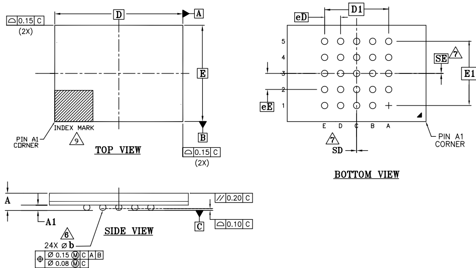
Figure 42. Ball Grid Array 24-Ball 6x8 mm (FAB024)
