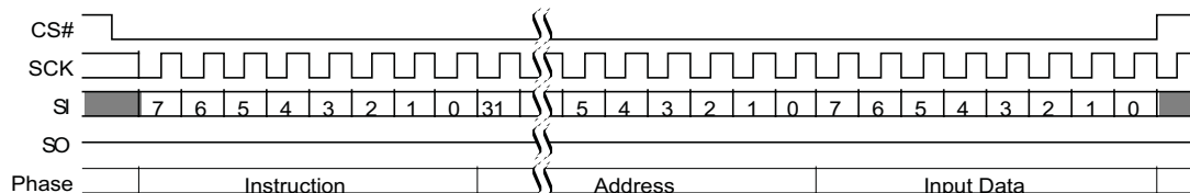
Figure 111. DYBWR (E1h) Command Sequence
