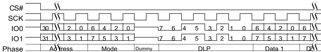
Figure 92. Continuous DDR Dual I/O Read Subsequent Access (4-Byte Address, EHPLC= 01b)
