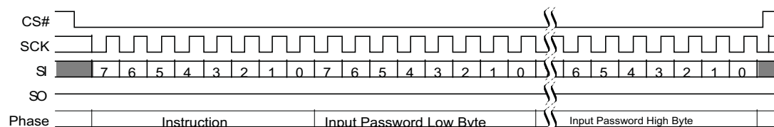
Figure 119. Password Unlock (PASSU E9h) Command Sequence
