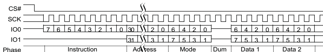
Figure 80. Dual I/O Read Command Sequence (4-Byte Address, BCh or BBh [ExtAdd=1], EHPLC=10b)
