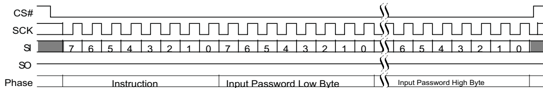
Figure 118. Password Program (PASSP E8h) Command Sequence
