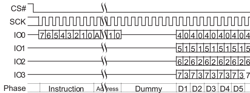
Figure 76. Quad Output Read (QOR 6Bh or 4QOR 6Ch) Command Sequence with Read Latency
