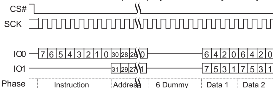
Figure 79. Dual I/O Read Command Sequence (4-Byte Address, BBh [ExtAdd=1], HPLC=10b)
