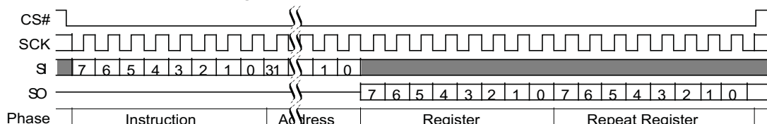
Figure 110. DYBRD Command Sequence
