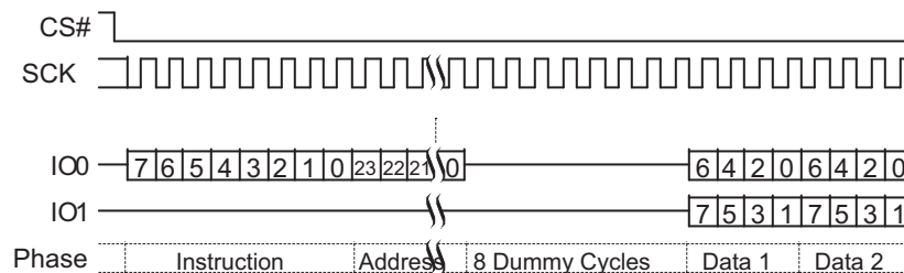
Figure 73. Dual Output Read Command Sequence (3-Byte Address, 3Bh [ExtAdd=0], LC=10b)
