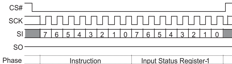
Figure 57. Write Registers (WRR 01h) Command Sequence – 8 data bits
