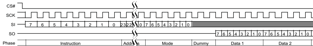
Figure 86. DDR Fast Read Initial Access (3-Byte Address, 0Dh [ExtAdd=0, EHPLC=11b])
