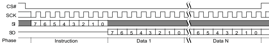
Figure 69. DLP Read (DLPRD 41h) Command Sequence
