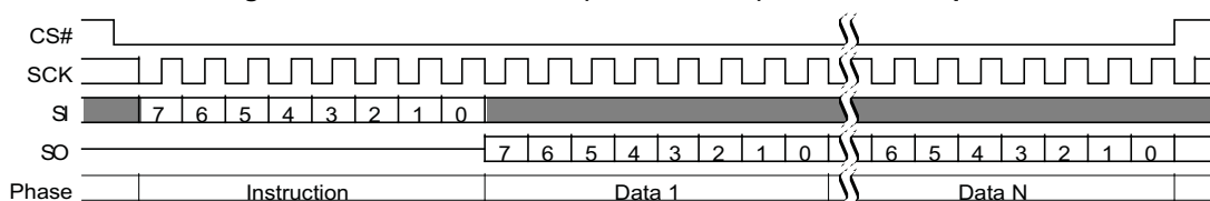
Figure 117. Password Read (PASSRD E7h) Command Sequence
