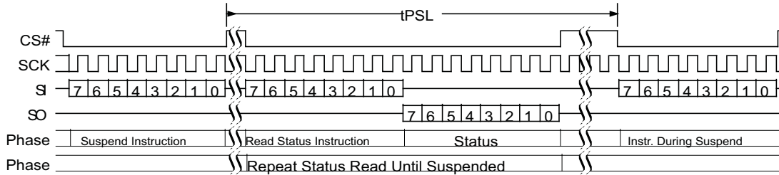
Figure 100. Program Suspend (PGSP 85h) Command Sequence
