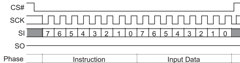
Figure 68. Write VDLR (WVDLR 4Ah) Command Sequence
