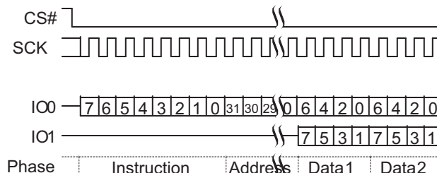
Figure 75. Dual Output Read Command Sequence (4-Byte Address, 3Ch or 3Bh [ExtAdd=1, LC=11b])
