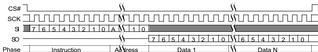
Figure 70. Read Command Sequence (READ 03h or 13h)
