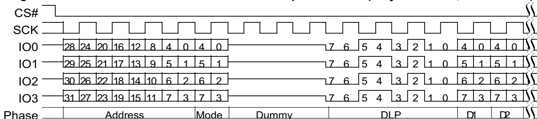
Figure 97. Continuous DDR Quad I/O Read Subsequent Access (4-Byte Address, EHPLC=01b)
