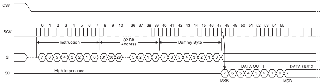
Figure 62. ECC Status Register Read Command Sequence
