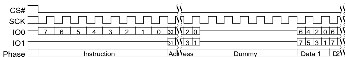
Figure 93. DDR Dual I/O Read (4-Byte Address, BEh or BDh [ExtAdd=1], HPLC=00b)
