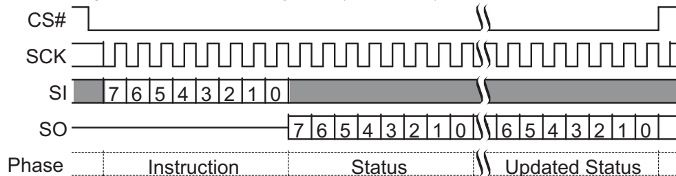
Figure 51. Read Status Register-1 (RDSR1 05h) Command Sequence
