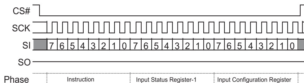
Figure 58. Write Registers (WRR 01h) Command Sequence – 16 data bits
