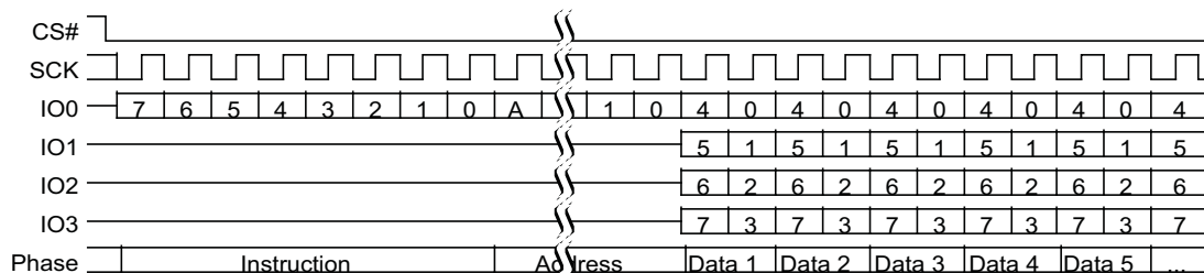
Figure 99. Quad 512-byte Page Program Command Sequence
