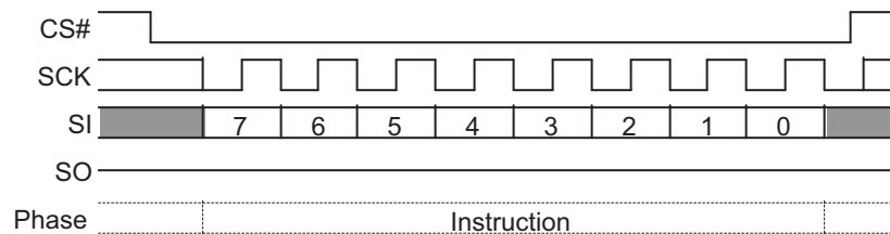
Figure 101. 10.55 Program Resume (PGRS 8Ah) Command Sequence
