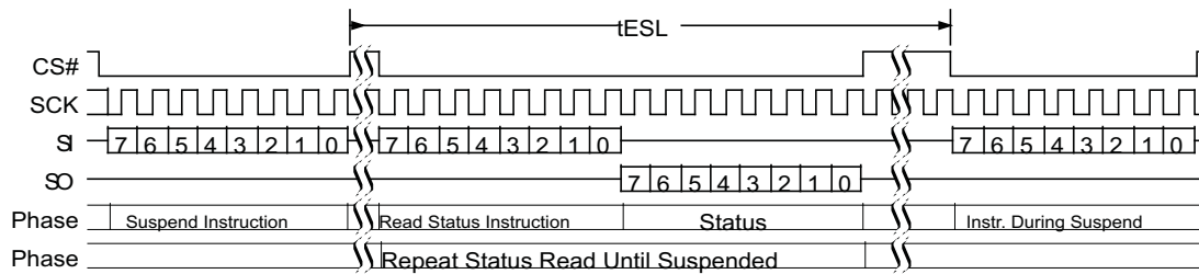
Figure 104. Erase Suspend (ERSP 75h) Command Sequence
