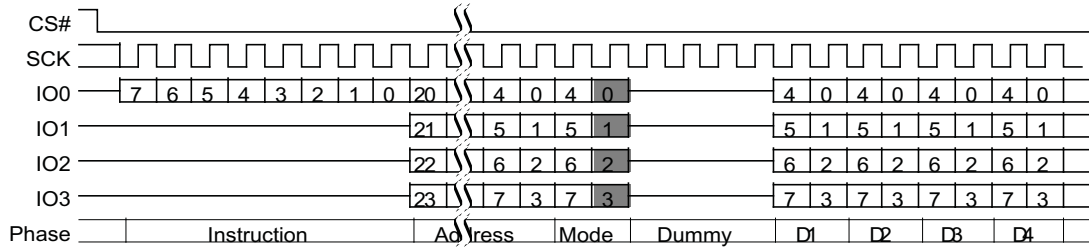
Figure 82. Quad I/O Read Command Sequence (3-Byte Address, EBh [ExtAdd=0], LC=00b)
