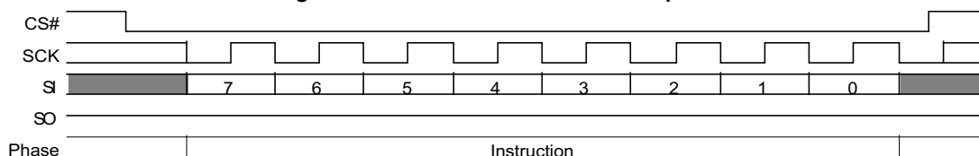
Figure 103. Bulk Erase Command Sequence
