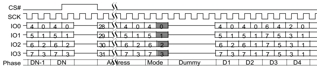
Figure 85. Continuous Quad I/O Read Command Sequence (4-Byte Address), LC=00b
