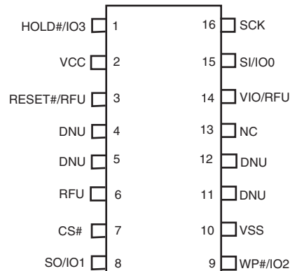
Figure 39. 16-Lead SOIC Package, Top View
