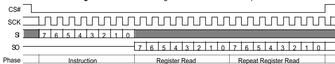
Figure 115. PPB Lock Register Read Command Sequence
