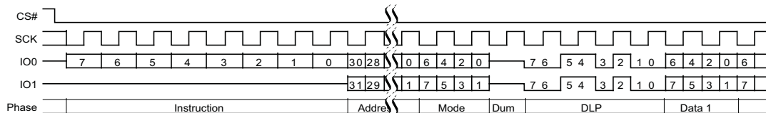
Figure 91. DDR Dual I/O Read Initial Access (4-Byte Address, BEh or BDh [ExtAdd=1], EHPLC= 01b)
