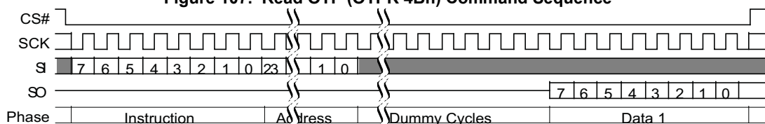
Figure 107. Read OTP (OTPR 4Bh) Command Sequence
