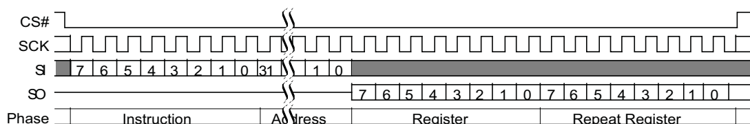
Figure 112. PPBRD (E2h) Command Sequence
