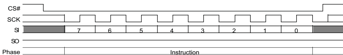
Figure 105. Erase Resume (ERRS 7Ah) Command Sequence
