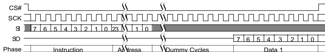
Figure 50. RSFDP Command Sequence
