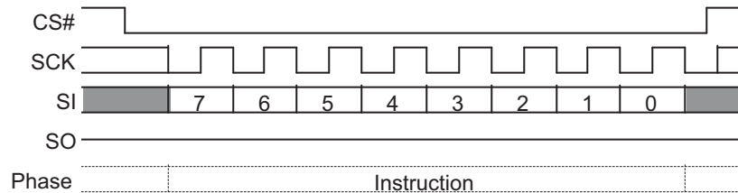
Figure 59. Write Enable (WREN 06h) Command Sequence
