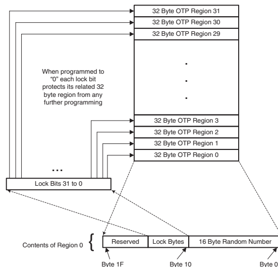
Figure 45. OTP Address Space
