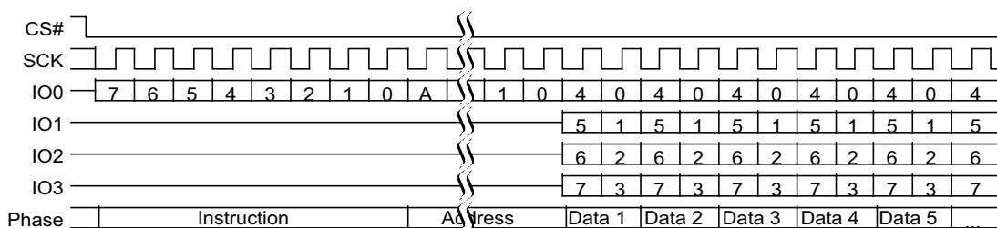
Figure 77. Quad Output Read (QOR 6Bh or 4QOR 6Ch) Command Sequence without Read Latency
