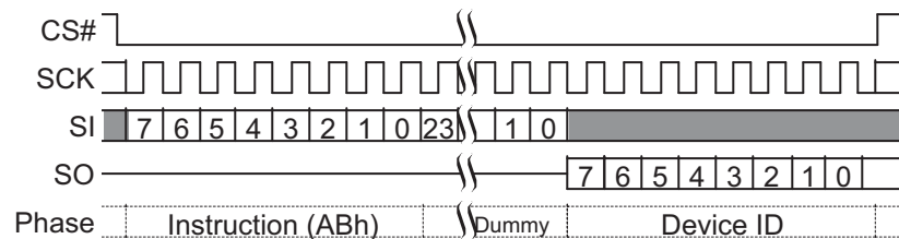
Figure 49. Read Electronic Signature (RES ABh) Command Sequence
