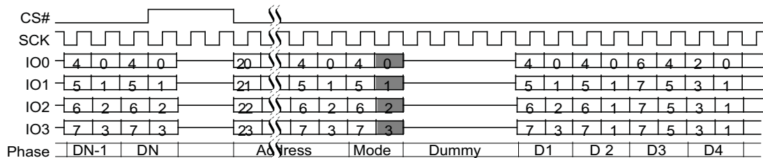
Figure 83. Continuous Quad I/O Read Command Sequence (3-Byte Address), LC=00b
