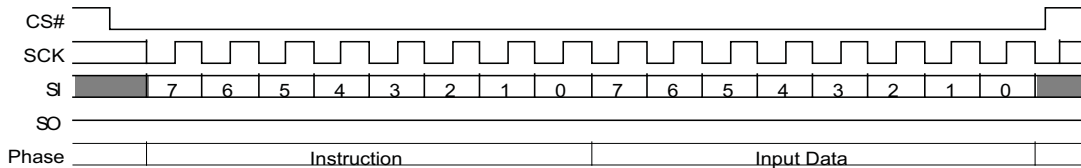
Figure 55. Bank Register Write (BRWR 17h) Command
