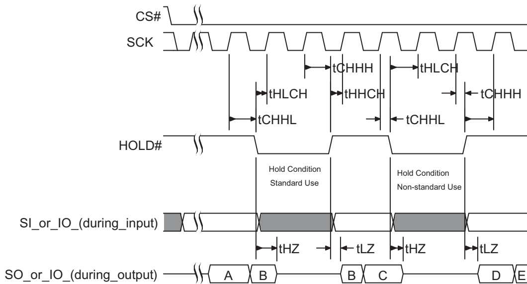
Figure 34. Hold Timing
