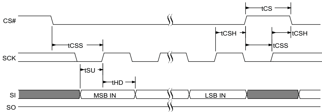
Figure 31. SPI Single Bit Input Timing
