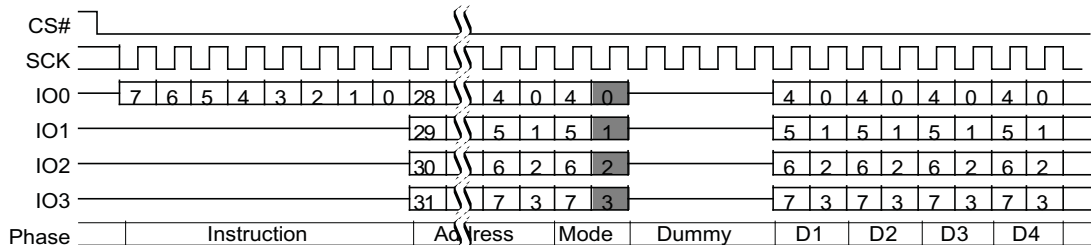
Figure 85. Continuous Quad I/O Read Command Sequence (4-Byte Address), LC=00b
