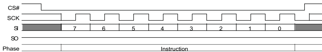
Figure 116. PPB Lock Bit Write (PLBWR A6h) Command Sequence
