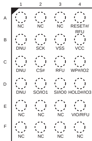
Figure 43. 24-Ball BGA, 4 x 6 Ball Footprint (FAC024), Top View
