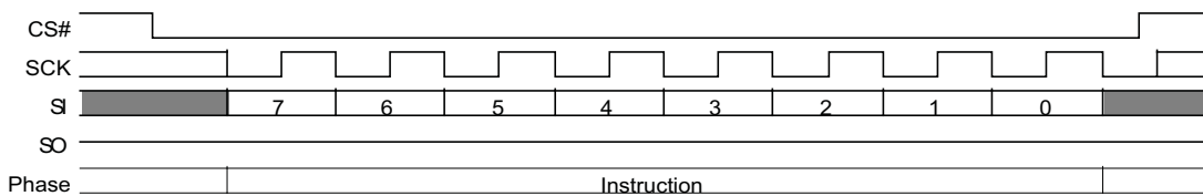
Figure 120. Software Reset (RESET F0h) Command Sequence
