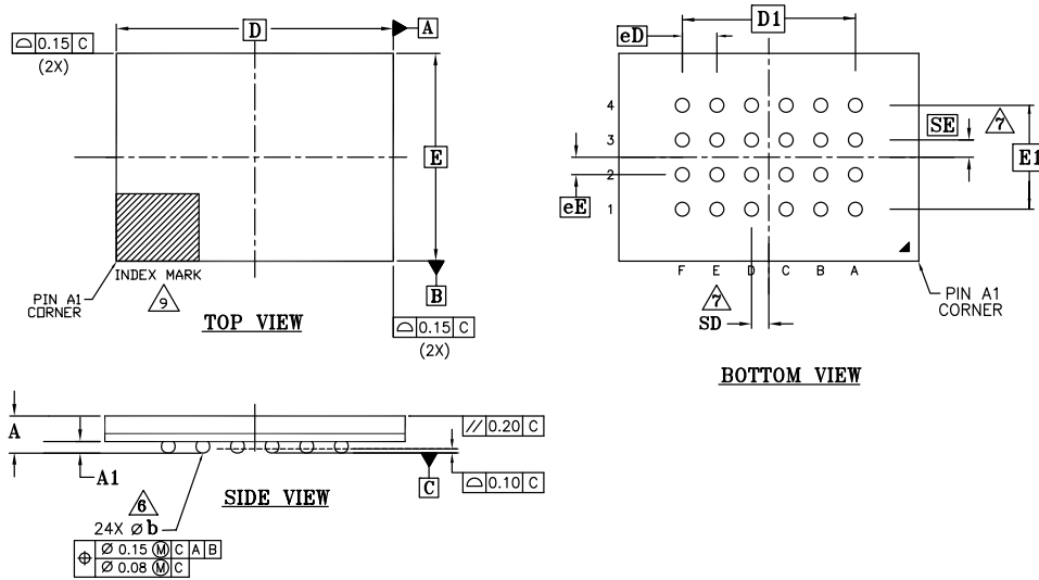
Figure 44. Ball Grid Array 24-Ball 6x8 mm (FAC024)
