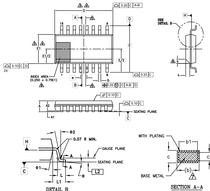
Figure 40. SOIC 16-Lead, 300-mil Body Width (SO3016)
