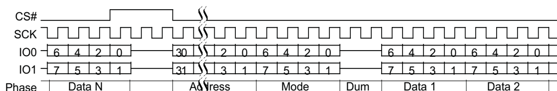
Figure 81. Continuous Dual I/O Read Command Sequence (4-Byte Address, BCh or BBh [ExtAdd=1], EHPLC=10b)
