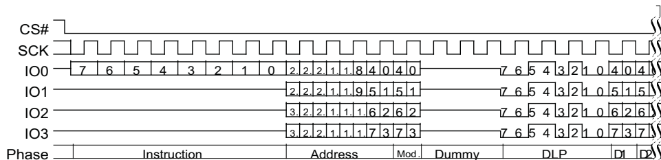
Figure 96. DDR Quad I/O Read Initial Access (4-Byte Address, EEh or EDh [ExtAdd=1], EHPLC=01b)
