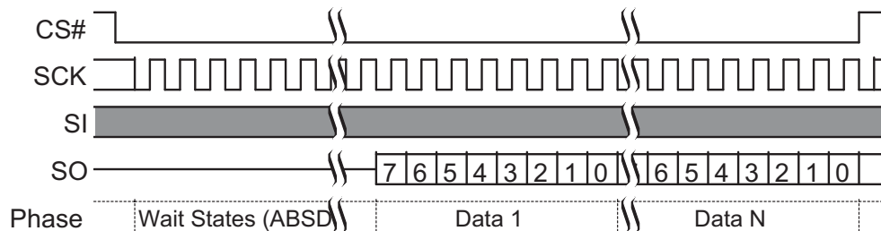
Figure 63. AutoBoot Sequence (CR1[1]=0)
