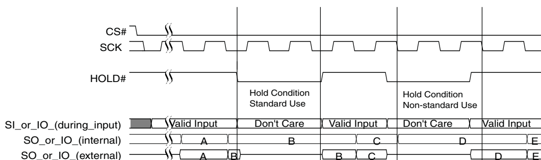
Figure 1. HOLD Mode Operation
