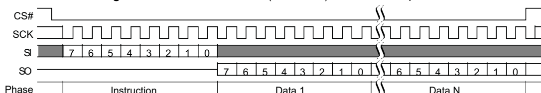
Figure 48. Read Identification (RDID 9Fh) Command Sequence
