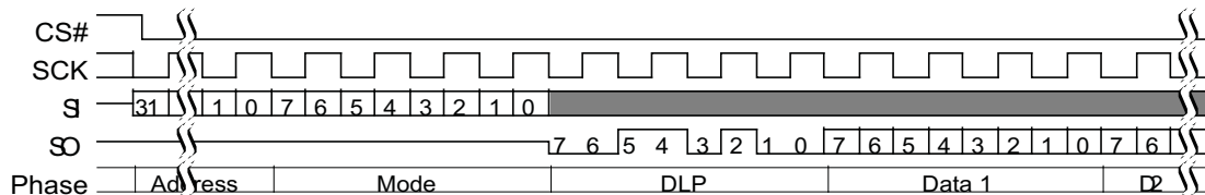
Figure 89. Continuous DDR Fast Read Subsequent Access (4-Byte Address [ExtAdd=1], EHPLC=01b)
