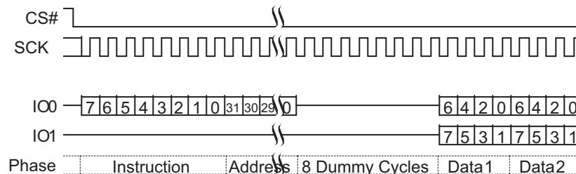
Figure 74. Dual Output Read Command Sequence (4-Byte Address, 3Ch or 3Bh [ExtAdd=1, LC=10b])
