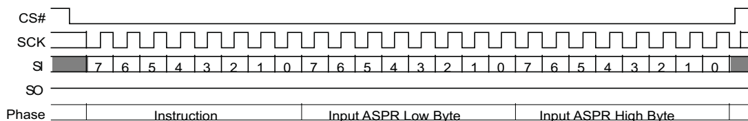
Figure 109. ASPP (2Fh) Command
