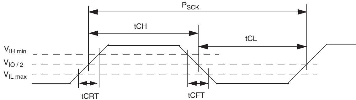
Figure 30. Clock Timing
