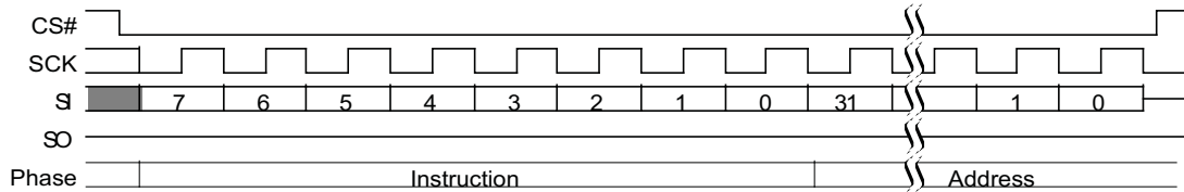
Figure 113. PPBP (E3h) Command Sequence
