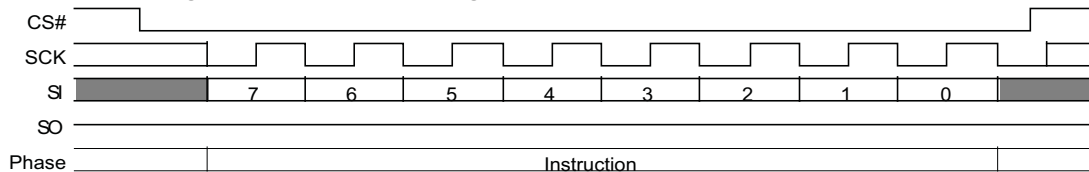
Figure 61. Clear Status Register (CLSR 30h) Command Sequence
