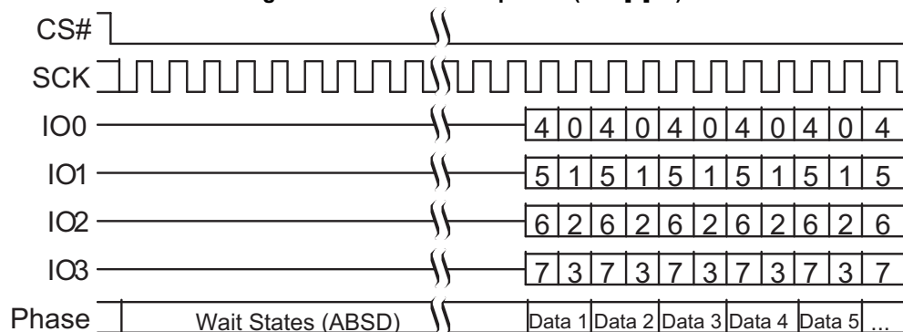
Figure 64. AutoBoot Sequence (CR1[1]=1)
