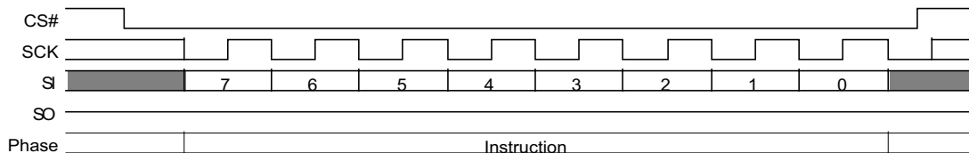
Figure 60. Write Disable (WRDI 04h) Command Sequence
