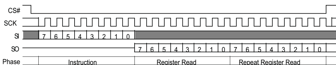
Figure 53. Read Configuration Register (RDCR 35h) Command Sequence
