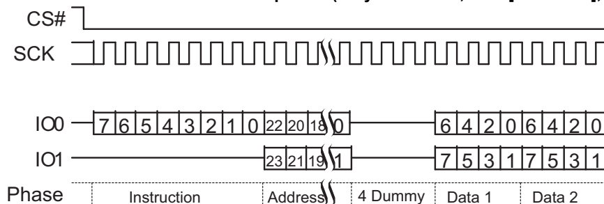
Figure 78. Dual I/O Read Command Sequence (3-Byte Address, BBh [ExtAdd=0], HPLC=00b)
