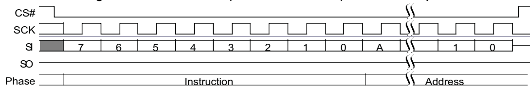
Figure 102. Sector Erase (SE D8h or 4SE DCh) Command Sequence
