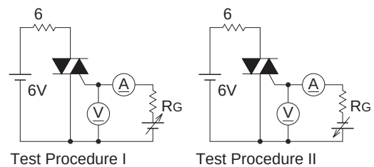
Gate Trigger Characteristics Test Circuits
