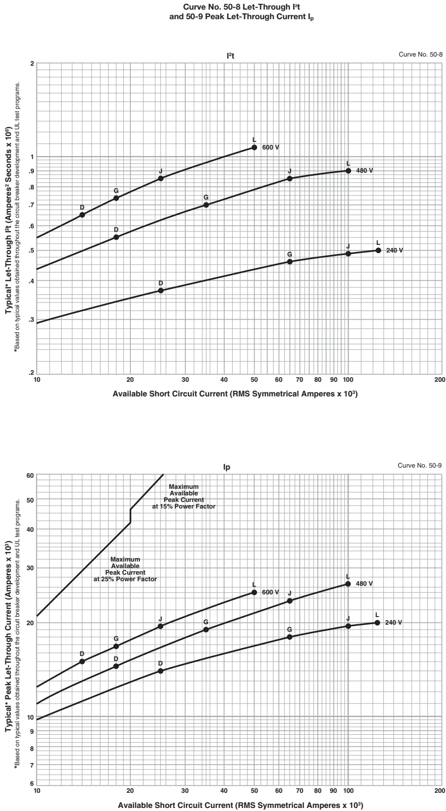
Figure 45: J-Frame 250 A (JD, JG, JJ, and JL)
