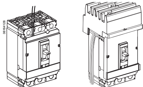
Figure 11: Accessory Connections
