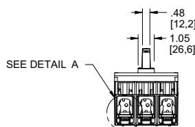
4896C-022-01 Top View Dimensions: Overall Width: 7.52 [191,0] Pin 1 to Pin 2: 6.22 [158,0] Pin 1 to Pin 3: 1.38 [35,0] Pin 1 to Pin 4: 1.30 [33,0] Pin 1 to Pin 5: 2.06 [52,4] Pin 1 to Pin 6: 1.38 [35,0] Pin 1 to Pin 7: 1.00 [25,5] Pin 1 to Pin 8: 1.76 [44,7] Pin 1 to Pin 9: 2.60 [66,1] Pin 1 to Pin 10: 5.57 [141,5] Pin 1 to Pin 11: 5.74 [145,8] Pin 1 to Pin 12: 6.52 [165,5] Pin 1 to Pin 13: 1.37 [34,8] Pin 1 to Pin 14: 4.12 [104,7] Pin 1 to Pin 15: 1.38 [35,0] Pin 1 to Pin 16: 0.20 [5,1] (MOUNTING HOLE) Side View Dimensions: Overall Height: 5.00 [127,0] Pin 1 to Pin 2: 3.44 [87,4] Pin 1 to Pin 3: 3.24 [82,4] Pin 1 to Pin 4: 2.87 [72,9] Pin 1 to Pin 5: 4.25 [108,0] Pin 1 to Pin 6: 1.91 [48,5] Pin 1 to Pin 7: 3.74 [95,1] Pin 1 to Pin 8: 19.9° OFF Pin 1 to Pin 9: 19.5° ON Pin 1 to Pin 10: 21.5° TRIPPED
