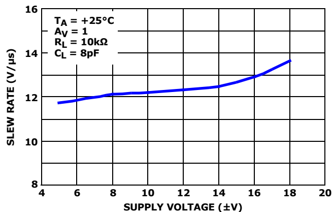
FIGURE 14. SLEW RATE vs SUPPLY VOLTAGE
