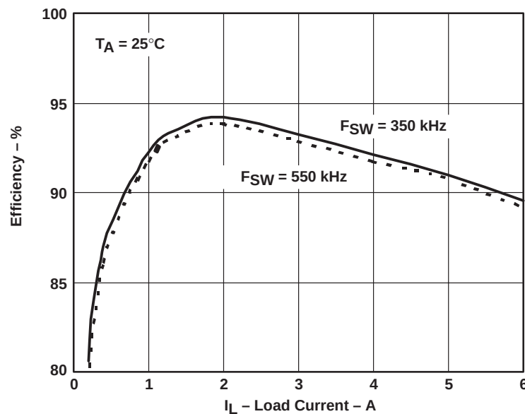
Figure 2–2. Measured Efficiency
