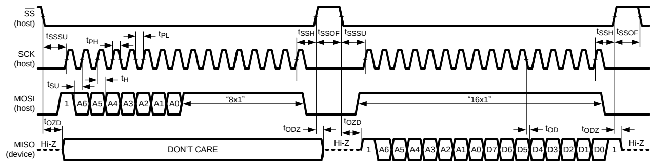
Figure 5. SPI Read
