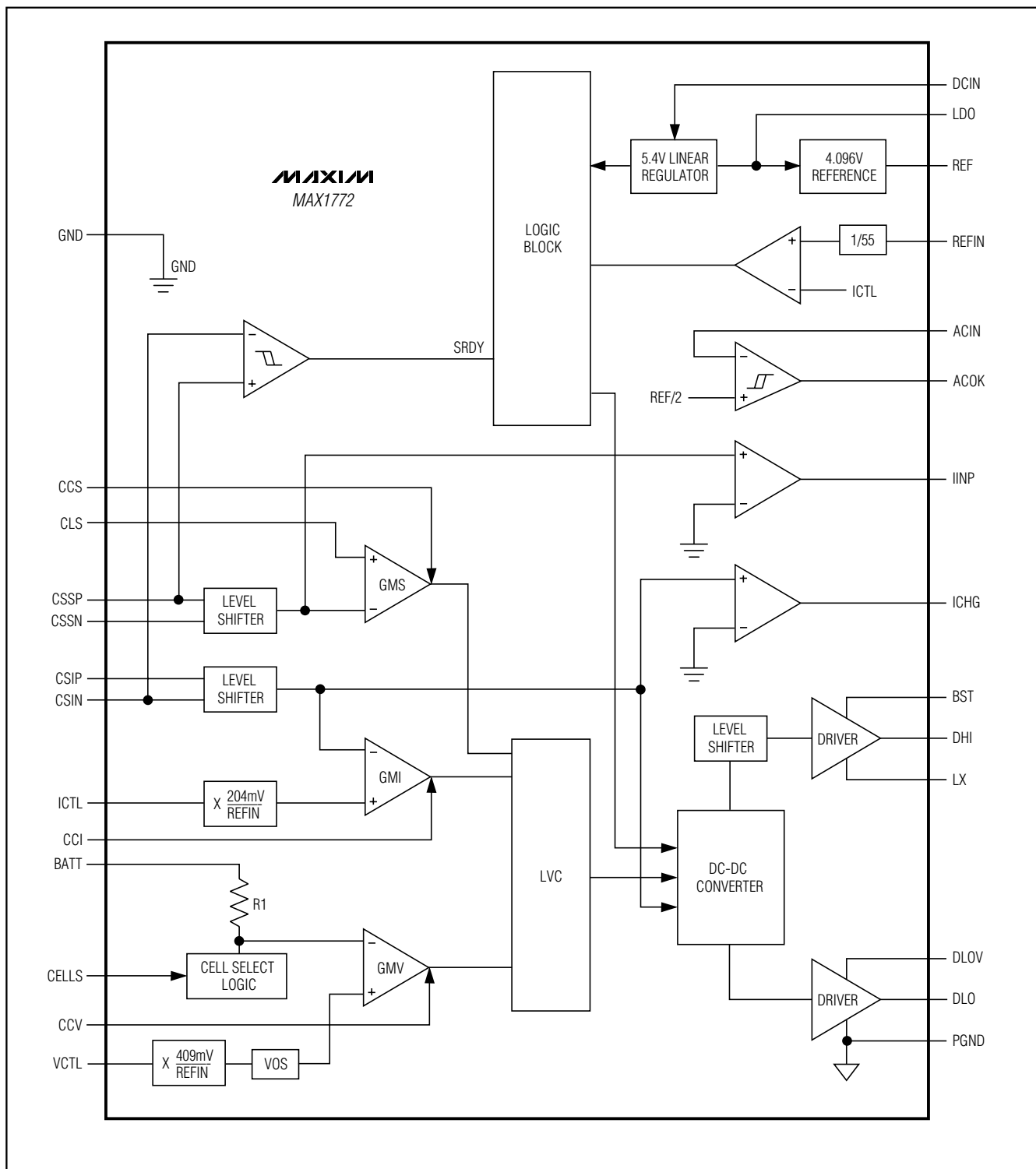
Figure 2. Functional Diagram
