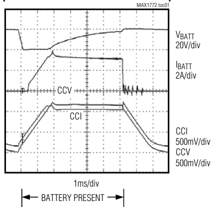
LOAD-TRANSIENT RESPONSE (BATTERY REMOVAL AND REINSERTION)
