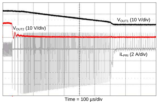
Figure 34. Secondary Short at I_{OUT2} = 600\text{mA} and I_{OUT1} = 200\text{mA}
