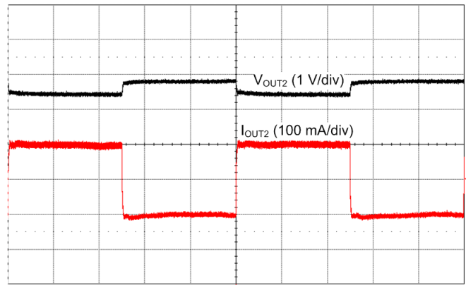
Figure 32. Load Transient at I_{OUT2} = 100\text{ mA} - 300\text{mA}
