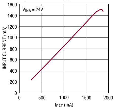
Input Current vs I_{\text{BAT}} , 18.8V Float
