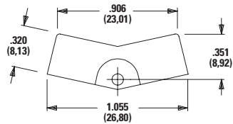
J3 Rocker
