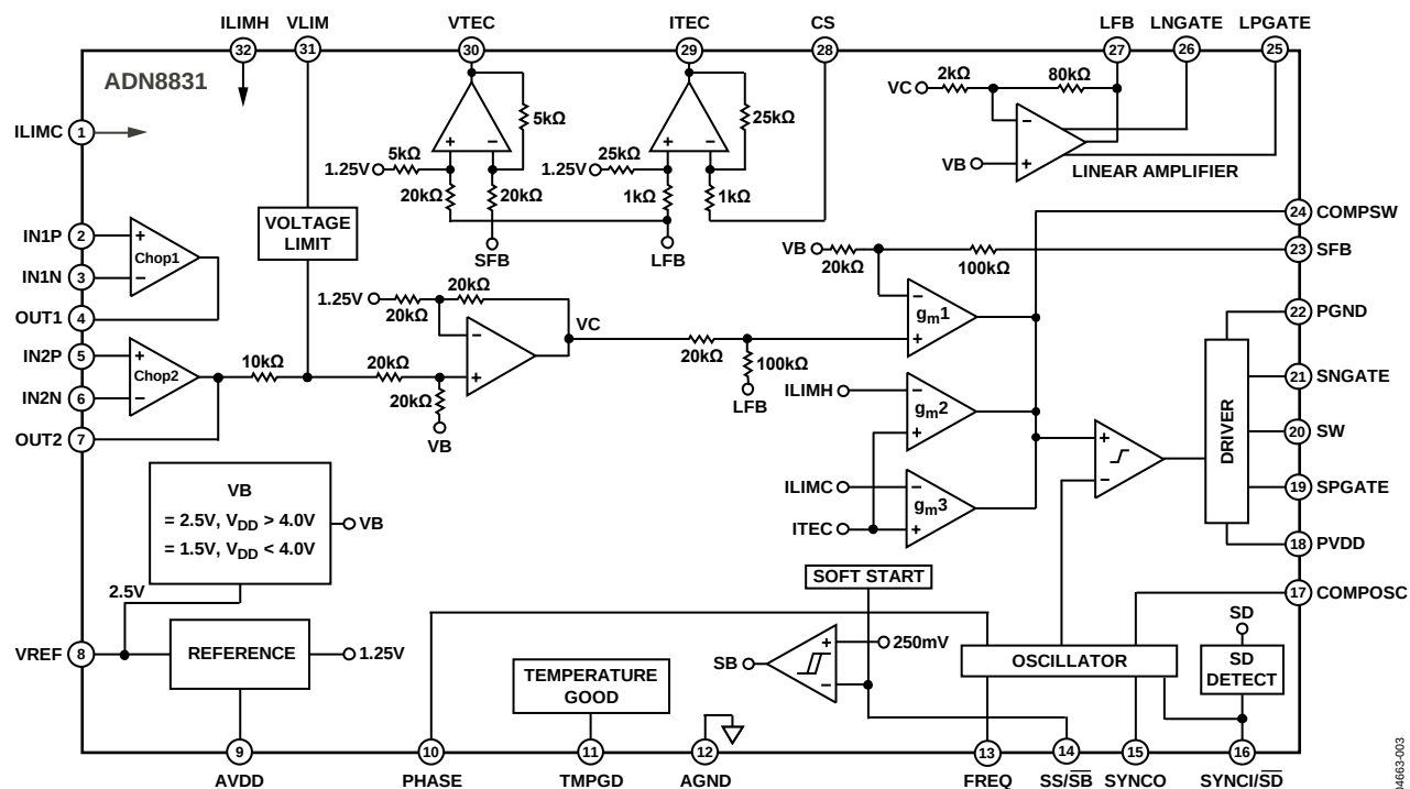
Figure 2. Detailed Block Diagram
