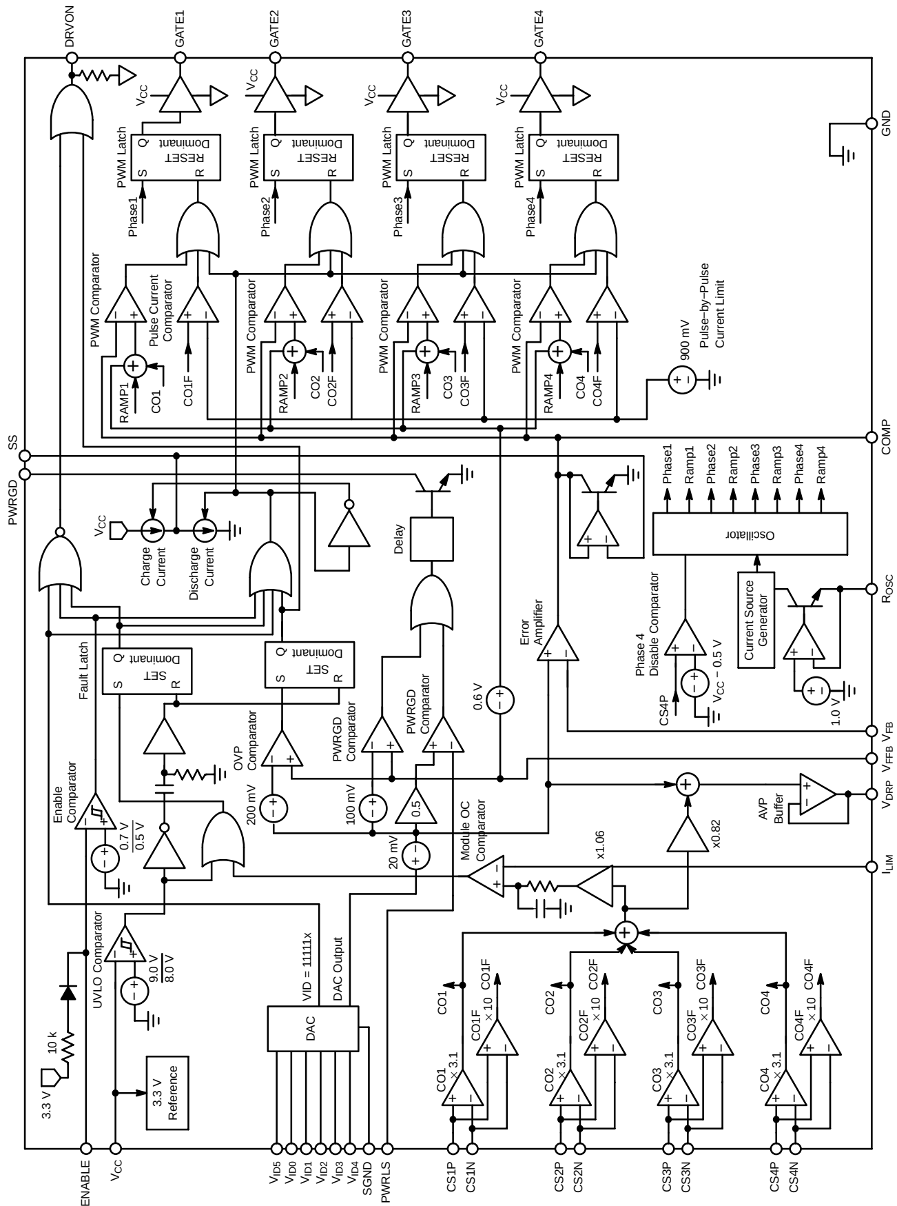
Figure 2. Block Diagram
