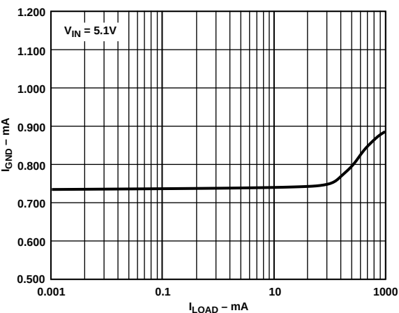
Figure 7. I_{GND} vs. I_{LOAD} ( V_{IN} = 5.1 V )*
