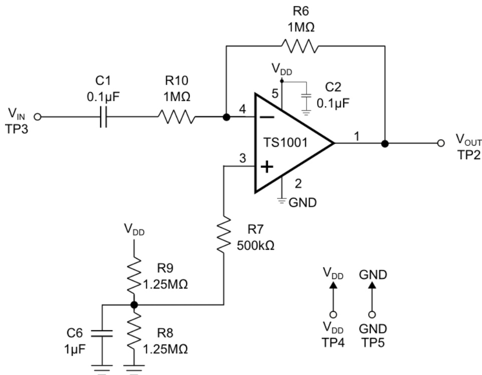
Figure 2. Inverting Configuration
