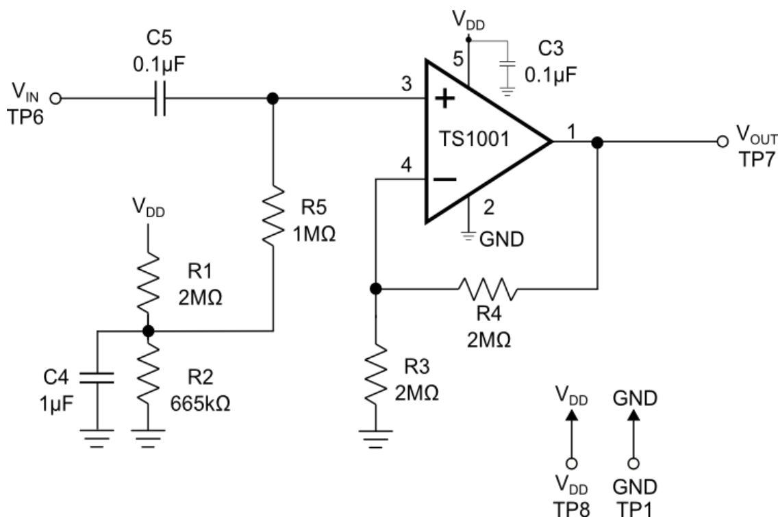
Figure 1. Non-Inverting Configuration
