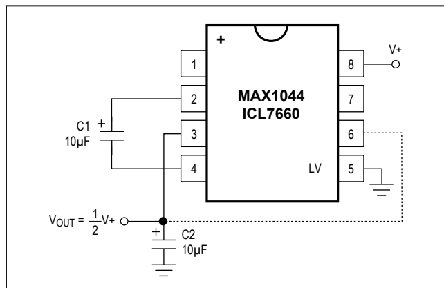
Figure 10. Voltage Divider
