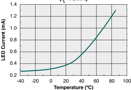
Typical I_F for Switch Operation ( I_L=70\text{mA} )
