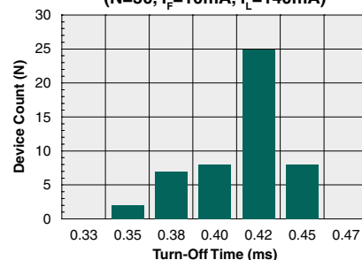
Typical Turn-Off Time (N=50, I_F=10\text{mA} , I_L=140\text{mA} )
