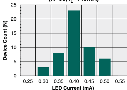
Typical I_F for Switch Operation (N=50, I_L=140\text{mA} )
