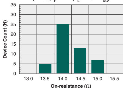
Typical On-Resistance Distribution (N=50, I_F=2\text{mA} , I_L=140\text{mA}_{DC} )
