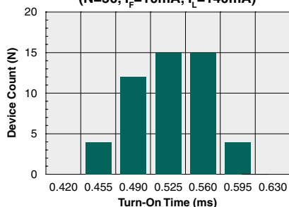
Typical Turn-On Time (N=50, I_F=10\text{mA} , I_L=140\text{mA} )
