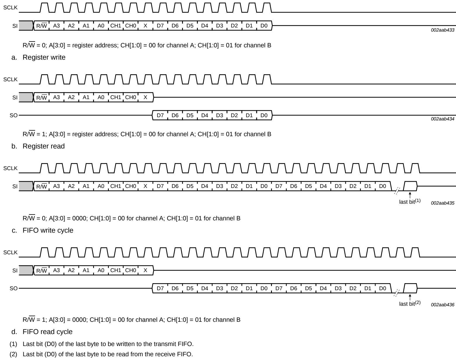
Fig 20. SPI operation
