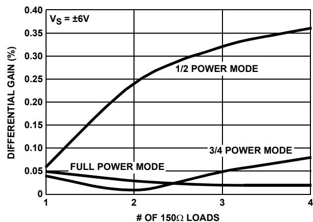
FIGURE 26. DIFFERENTIAL GAIN
