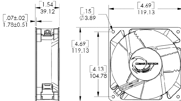
MECHANICAL DRAWING
