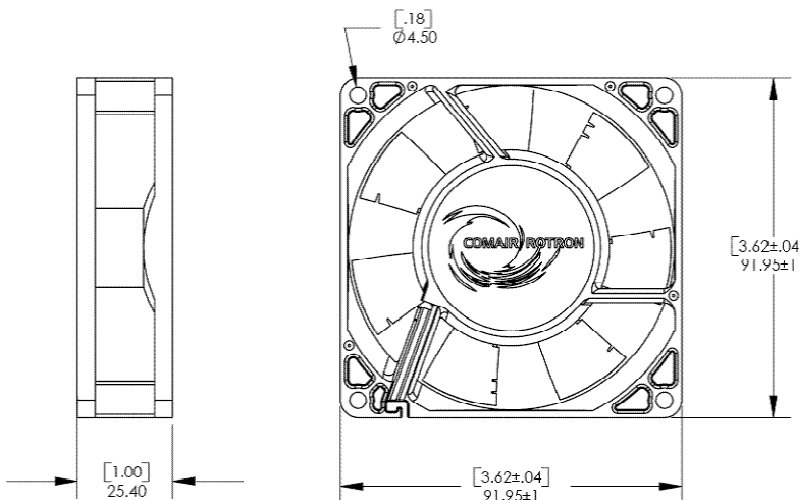
MECHANICAL DRAWING
