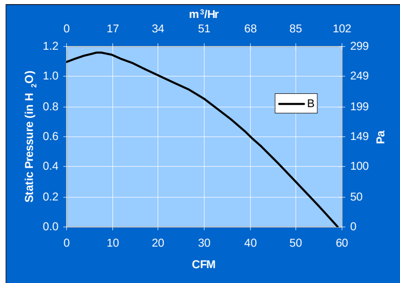
PERFORMANCE GRAPH
