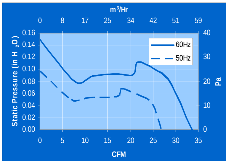
PERFORMANCE GRAPH
