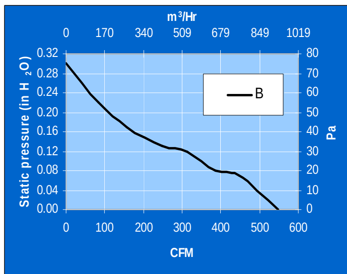
PERFORMANCE GRAPH
