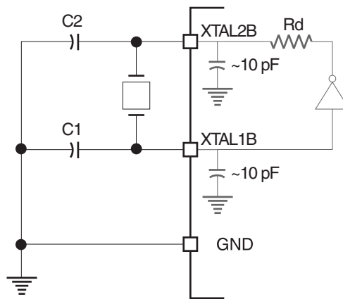
Figure 6-5. Crystal Oscillator B Connections
