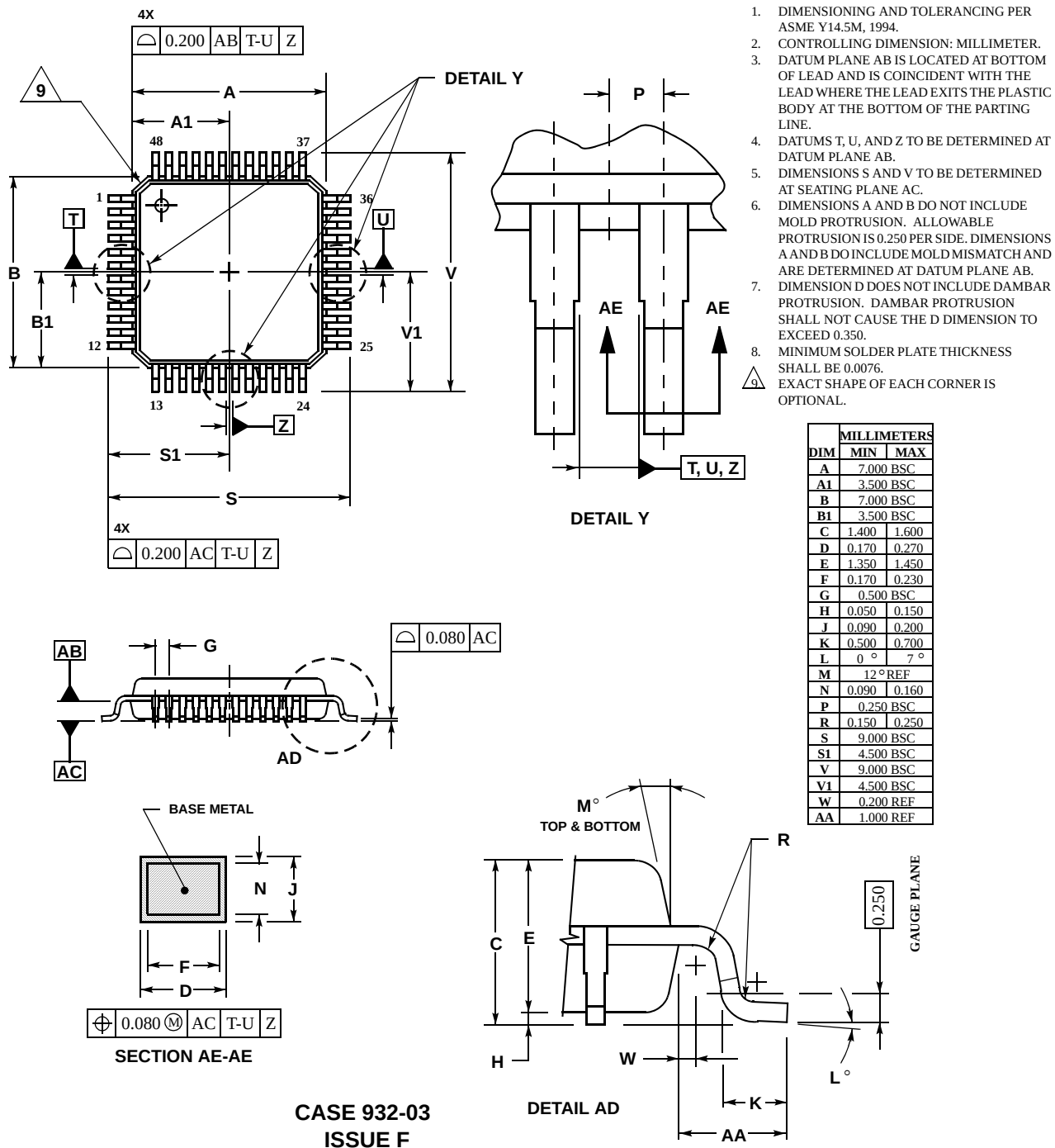
Figure 4-2 48-pin LQFP Mechanical Information
