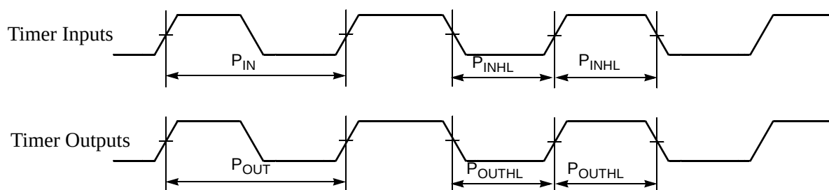
Figure 3-23 Timer Timing
