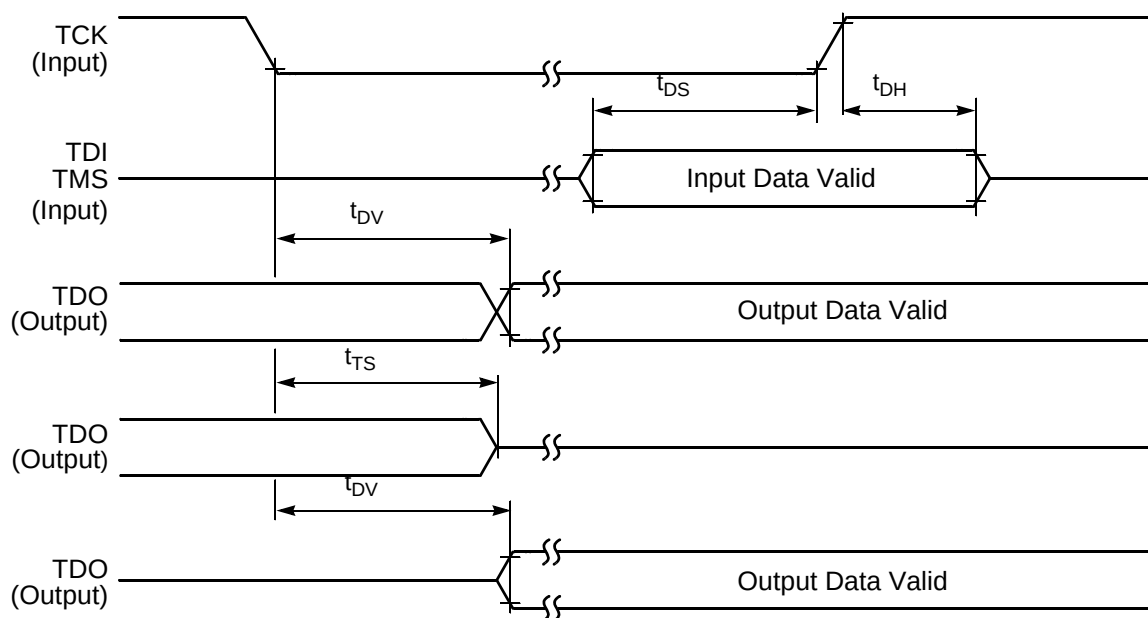
Figure 3-28 Test Access Port Timing Diagram
