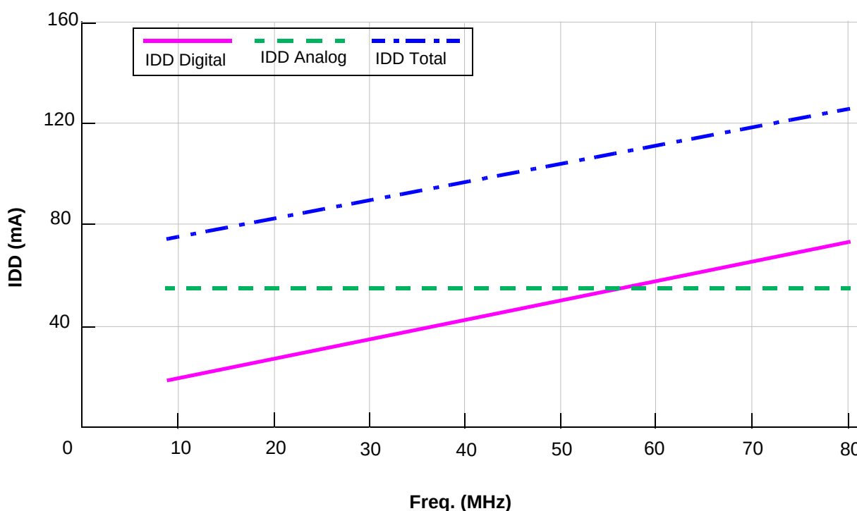
Figure 3-1 Maximum Run IDD vs. Frequency (see Note 7. in Table 3-15)
