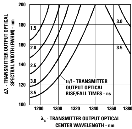
HFBR-5903 FDDI TRANSMITTER TEST RESULTS OF \lambda_c , \Delta\lambda AND tr/\tau ARE CORRELATED AND COMPLY WITH THE ALLOWED SPECTRAL WIDTH AS A FUNCTION OF CENTER WAVELENGTH FOR VARIOUS RISE AND FALL TIMES.
