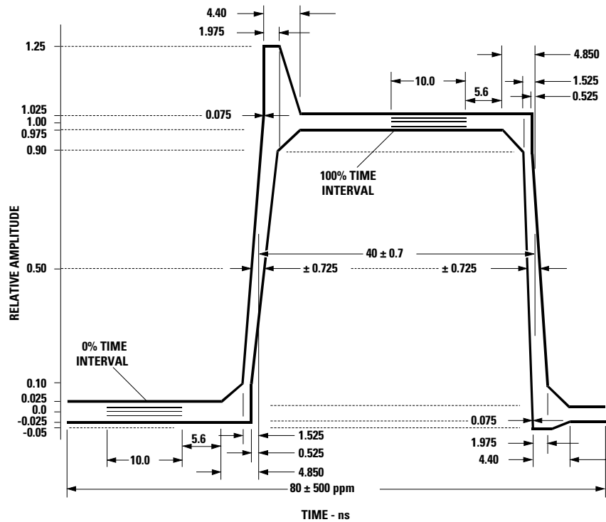
THE HFBR-5903 OUTPUT OPTICAL PULSE SHAPE SHALL FIT WITHIN THE BOUNDARIES OF THE PULSE ENVELOPE FOR RISE AND FALL TIME MEASUREMENTS.
