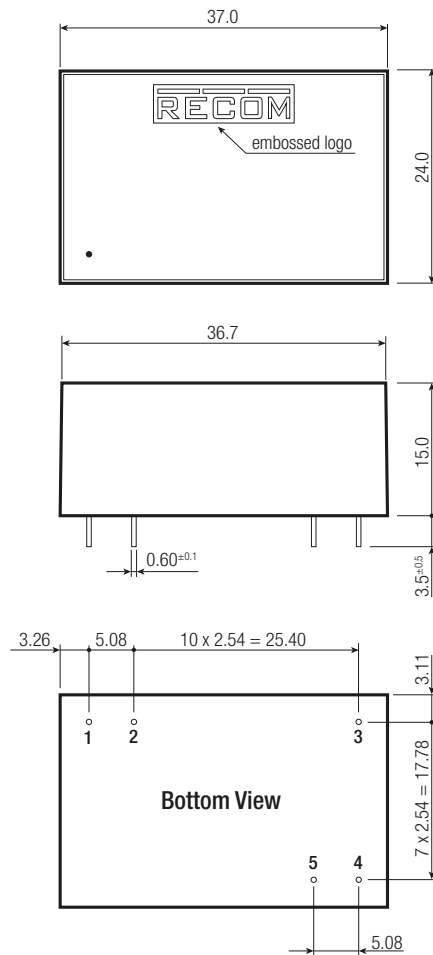
Dimension Drawing (mm)
