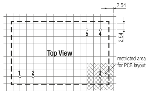
Recommended Footprint Details
