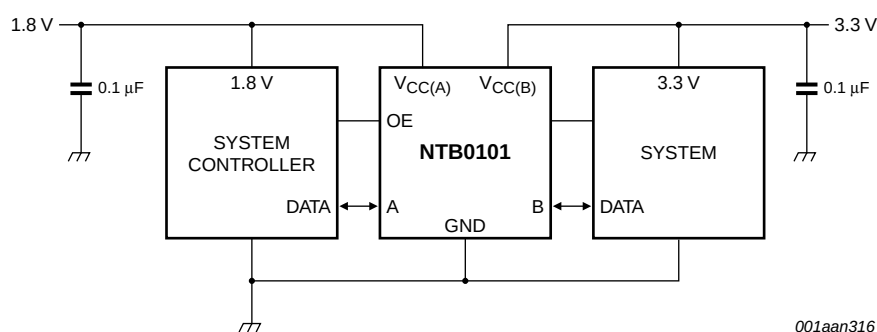
Fig 8. Typical operating circuit
