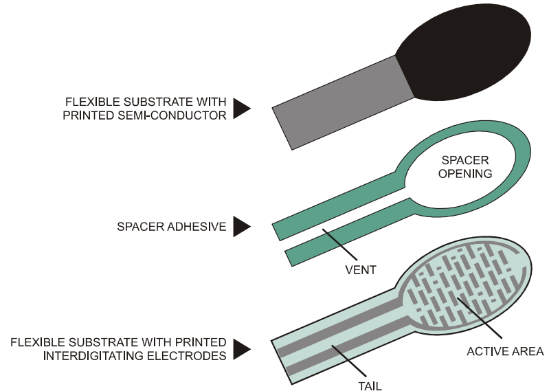
Figure 1: FSR Construction
