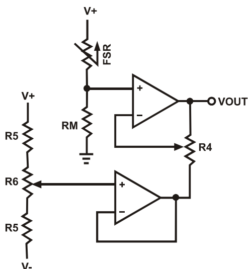
Figure 11 Adjustable Buffer
