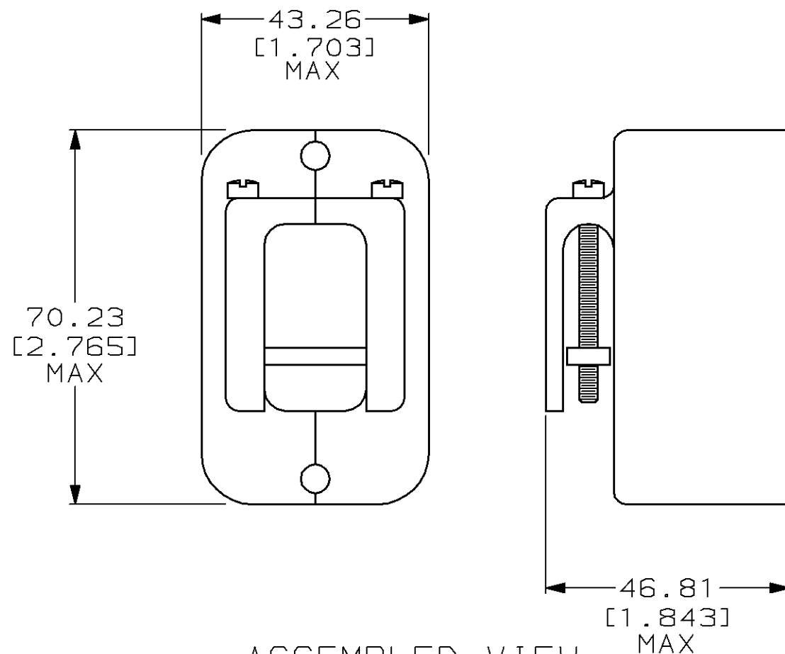
ASSEMBLED VIEW
