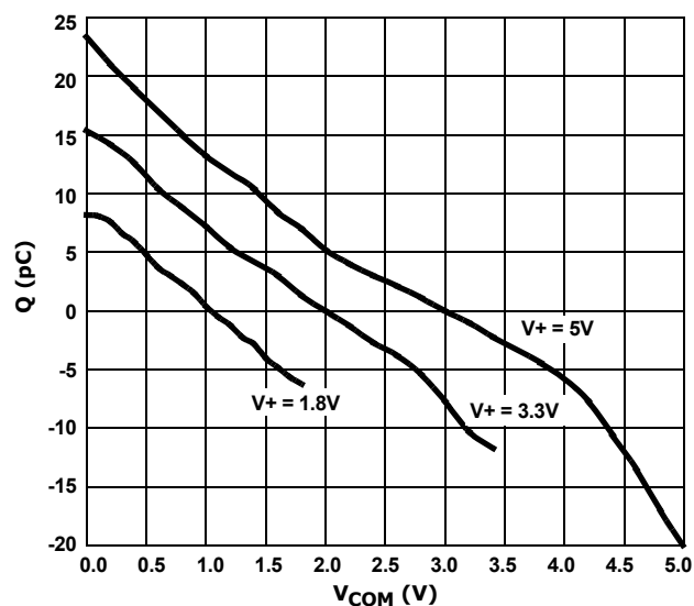
FIGURE 19. CHARGE INJECTION vs SWITCH VOLTAGE
