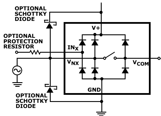
FIGURE 9. OVERVOLTAGE PROTECTION
