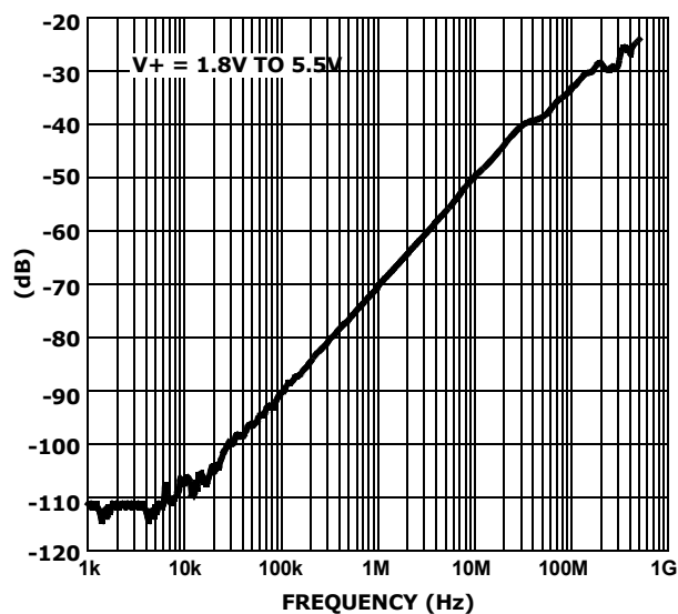
FIGURE 18. OFF-ISOLATION
