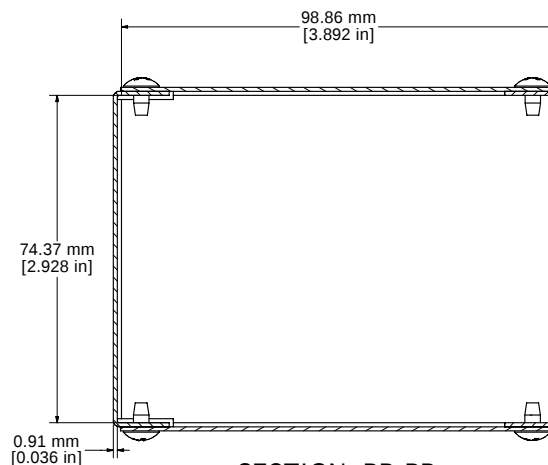
SECTION BB-BB
