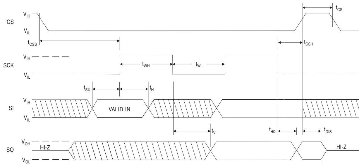
Figure 4-1. Synchronous Data Timing
