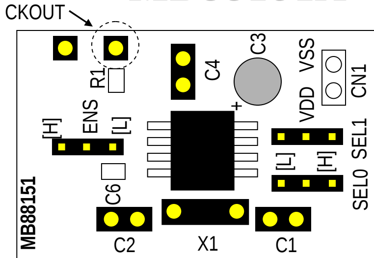
Fig. MB88151AEB01-xxx
