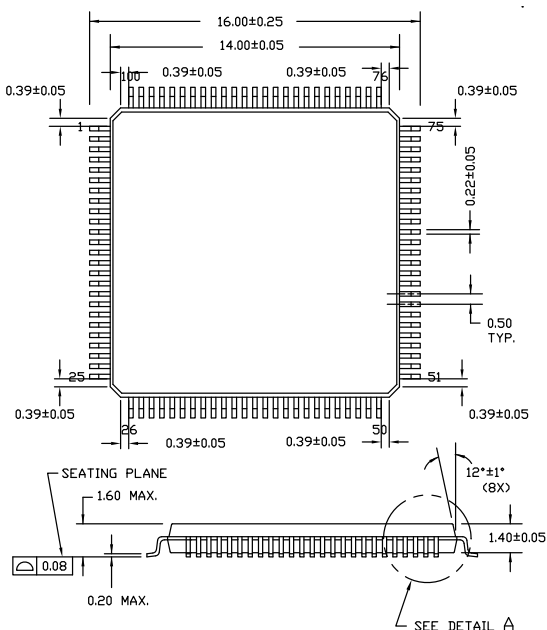
Figure 16. 100-pin TQFP (14 × 14 × 1.4 mm) A100SA Package Outline, 51-85048
