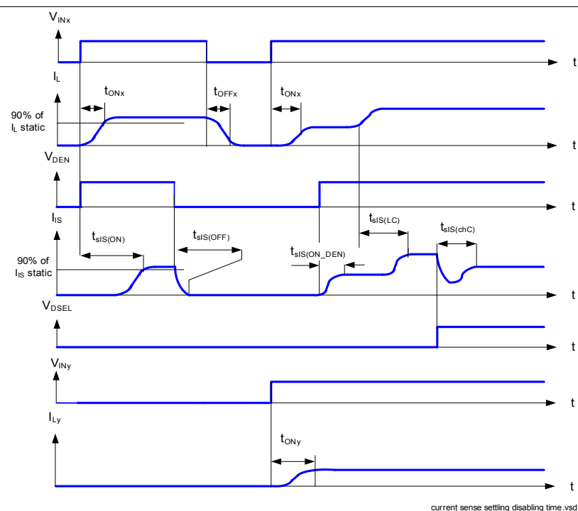
Figure 23 SENSE Settling / Disabling Timing
