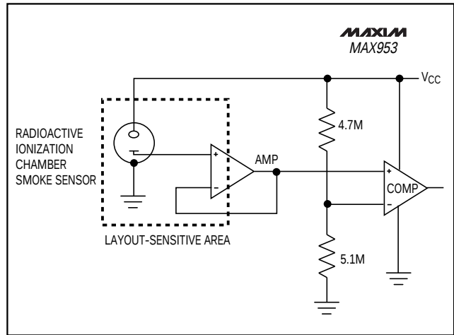
Figure 6. Sensor Preamplifier and Alarm Trigger Application
