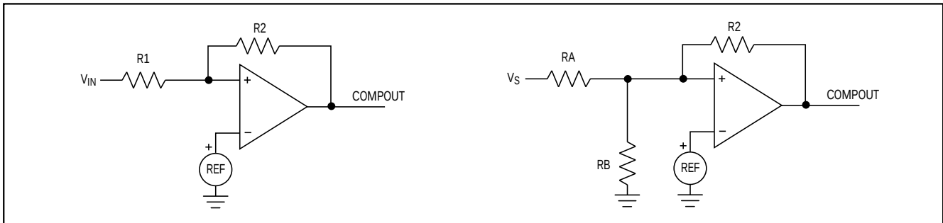
Figure 2. External Hysteresis
