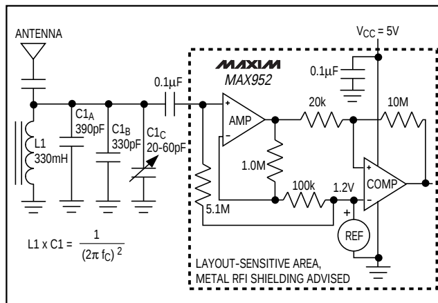
Figure 4. Low-Frequency Radio Receiver Application
